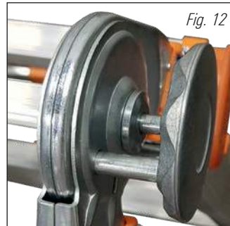
Fig. 12 Unlocked joint
