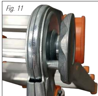
Fig. 11 Locked joint
